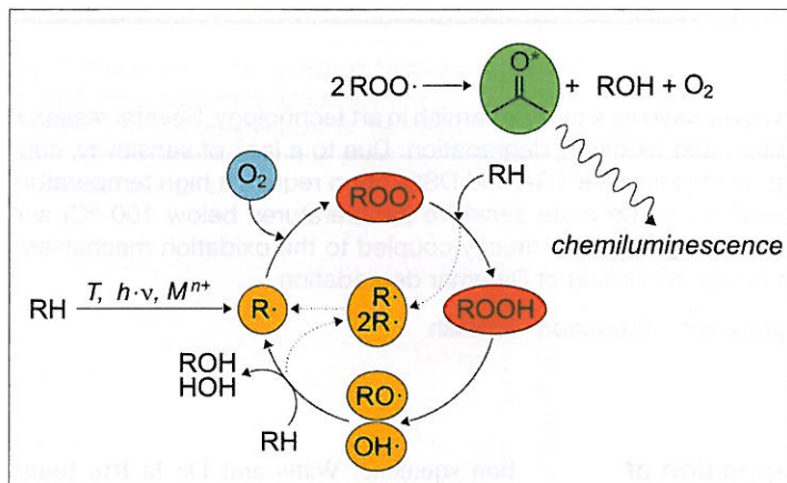
Fig. 3. Autooxidation cycle and the recombination process generating chemiluminescence (Russell mechanism)
