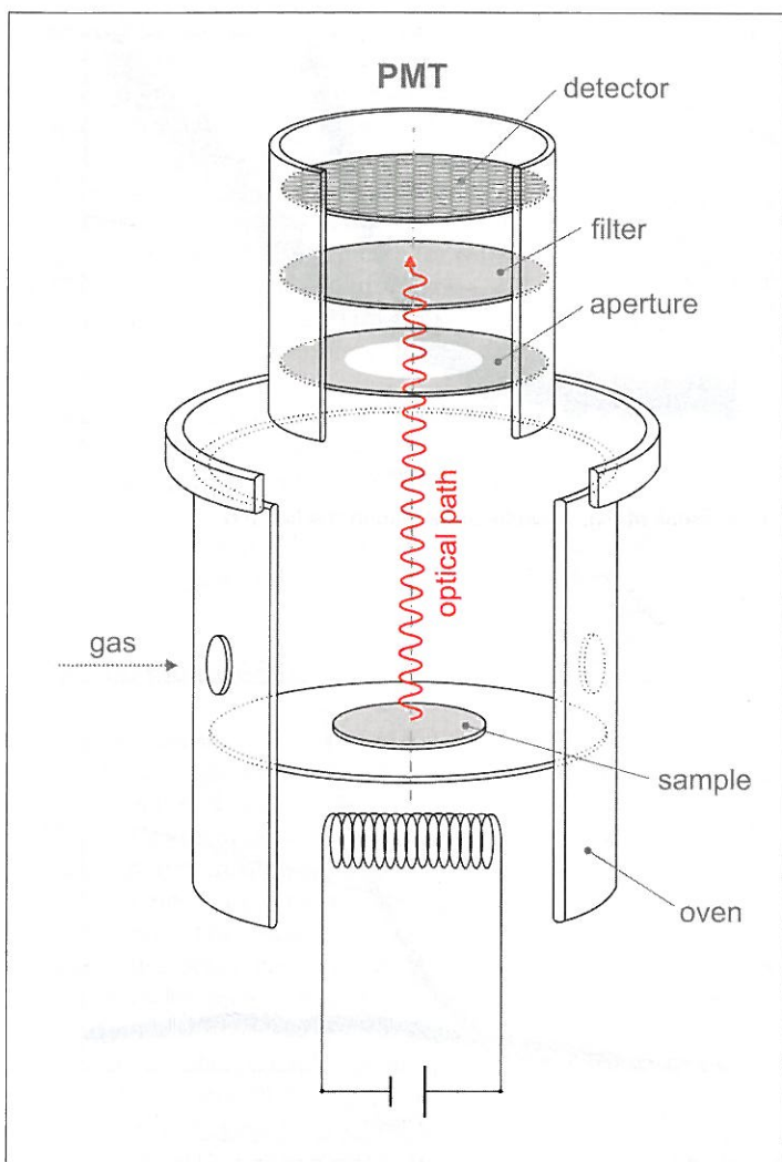
Fig. 4. Scheme of the chemiluminescence measuring device
