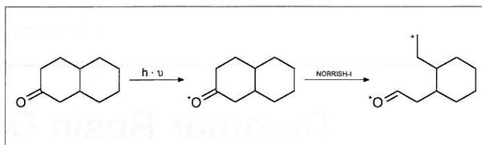
Scheme 1. Norrish-I ring cleavage
