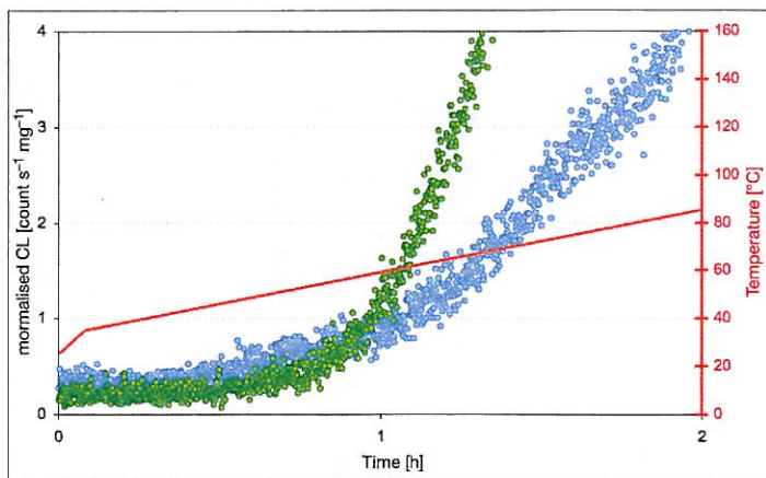
Fig. 8. Detail of Fig. 7: signal onset during the first 2 h
