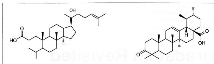
Fig. 2. Examples of triterpenoid structures: dammarenolic acid (left) and ursonic acid (right)
