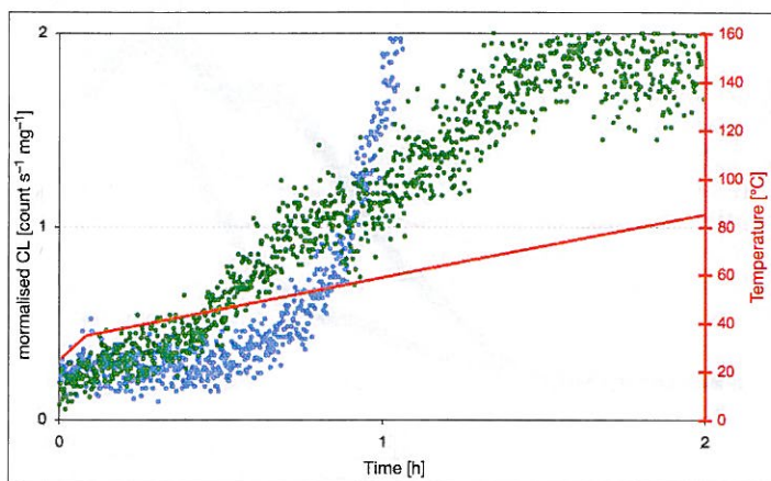
Fig. 6. Detail of Fig. 5: signal onset during the first 2 h
