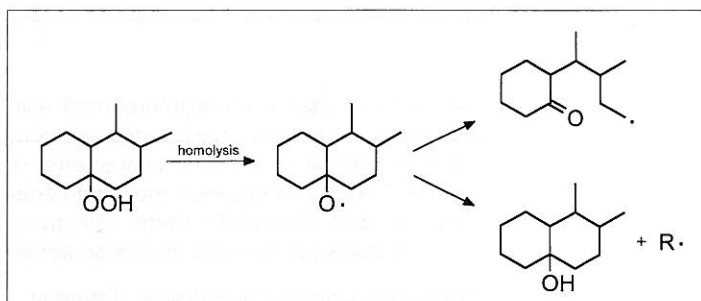
Scheme 2. Alkyl radicals forming new polar functional groups
