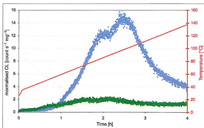
Fig. 5. Chemiluminescence signals of dammar samples taken from the surface (blue curve) and the inner (green curve) regions of a raw dammar lump. Measurement in pure nitrogen in the range from 308 to 413 K at a heating rate of 0.44 K/min.
