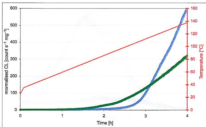
Fig. 7. Chemiluminescence signals of dammar samples taken from the surface (blue curve) and the inner (green curve) regions of a raw dammar lump. Measurement in pure oxygen in the range from 308 to 413 K at a heating rate of 0.44 K/min.
