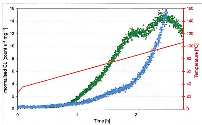
Fig. 9. Chemiluminescence signal onset (2.8 h) of dammar samples taken from the surface of a raw dammar lump. Measurements in pure oxygen (blue curve) and in pure nitrogen (green curve).
