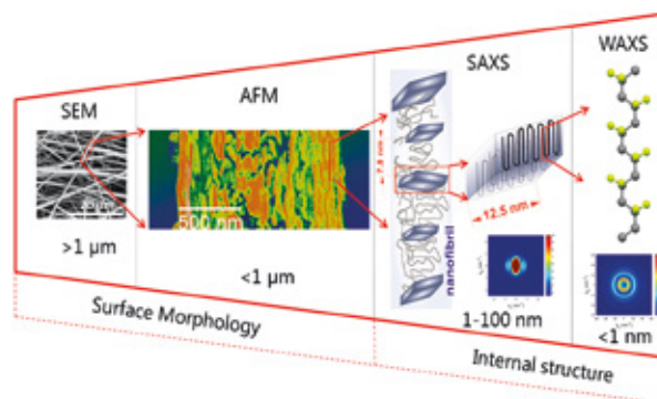
Schematic representation of the multimodal and multidimensional analytical approach for electrospun PVDfHfp fibers: from nanofiber morphology to the atomic structure.
