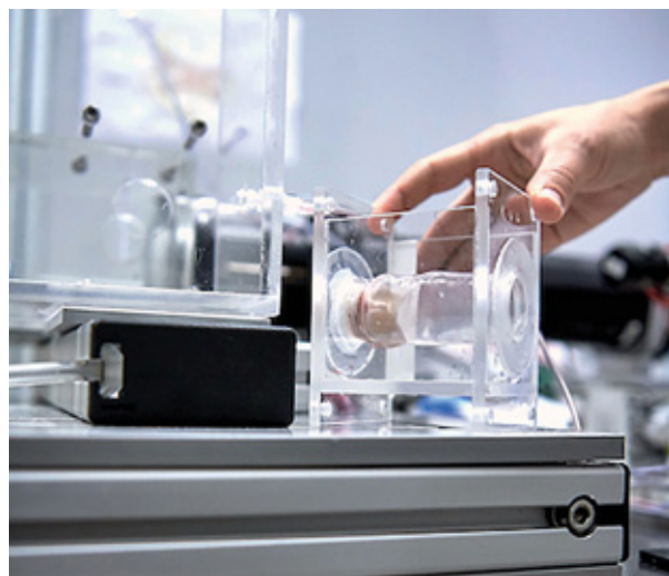
Bioprosthesis heart valve in a test cell
