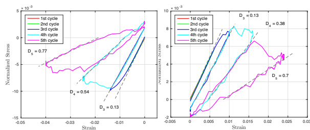
Cyclic normalised stress-strain curves for trabecular bone in compression and tension using explicit finite element analysis
