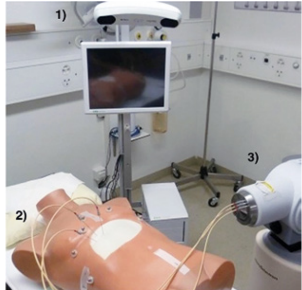
Experimental setup showing the navigation system 1), the phantom 2), and the brachytherapy system 3).
