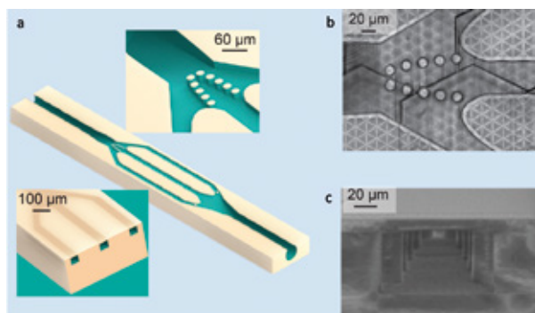
(a) Schematic CAD visualization of the microchannel used to trap a single C. elegans worm. (b) Optical microscope image and (c) SEM image of a 3D printed section of the trapping system inside the microchannel. Collaboration with Prof. J. Brugger, EPFL.
