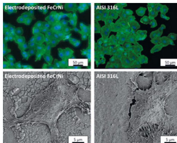
Cytotoxicity tests: A comparison of cell adhesion (top pictures) and morphology (bottom pictures) on electrodeposited Fe-Cr-Ni and AISI 316L stainless steel.
