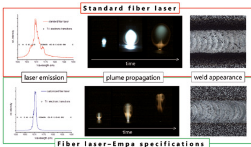
High speed camera side views, SEM weld pictures
