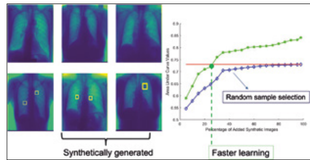
Focused Active Learning. Exploiting sample informativeness and synthetic data augmentation enables a faster learning (see slope of green curve) versus standard active-learning approaches (blue curve), and an improved use of the information compared to the performance obtained when training with all available data at once (red line)
