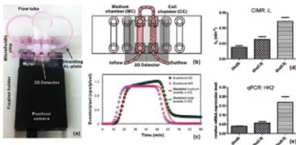
The continuously infused microfluidic radioassay (CIMR) system: (a) photograph of the microfluidic chip in operation; (b) sketch of the tracer medium flow during the measurement; (c) representative cellular pharmacokinetic modelling; (d,e) comparison of cellular pharmacokinetics with relevant qPCR results for human breast cancer cell line SkBr3 cultured in media of three different glucose concentrations (0.5, 2.5, and 5 mM).
