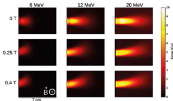
Measured dose distributions for electron beams with different energies and for different magnetic field strengths.
