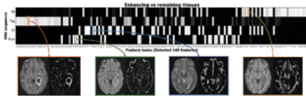
Global interpretability of deep learning features to segment enhancing tissue. Features are sorted from most to least important (left to right). Brighter means higher squared L2-norm of the weights connecting the hidden unit of a given feature to a given MRI sequence. Bottom) examples of pairs of MRI sequences (left) and feature maps (right). Source: Pereira et al. Medical Image Analysis , 2018.
