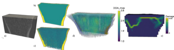
HR-pQCT image (a) with segmentation of cortex (b) and trabeculae (c) to extract main orientation or fabric (d) and finite element analysis to estimate failure load of the wrist
