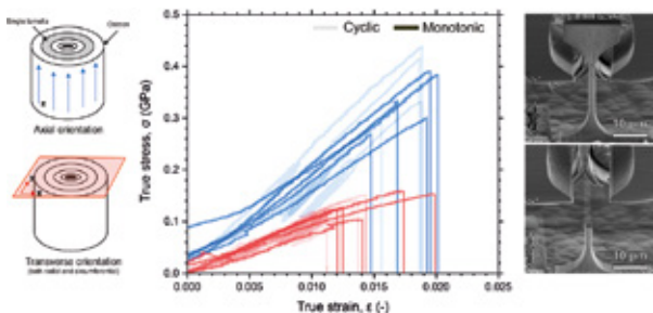
Micro-tensile stress strain behavior of ovine osteonal bone (left), high resolution secondary electron image of a micro-tensile specimen before and after loading (right)
