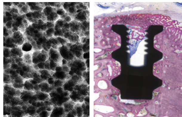
The ufgTi viewed in the laser confocal microscope (left). Excellent osseointegration after 8 weeks (right).
