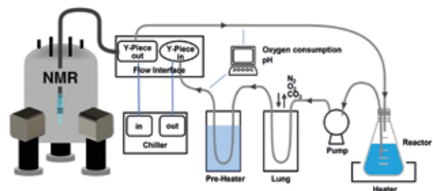
Bioreactor for online Metabolomics of living cells inside the NMR.
