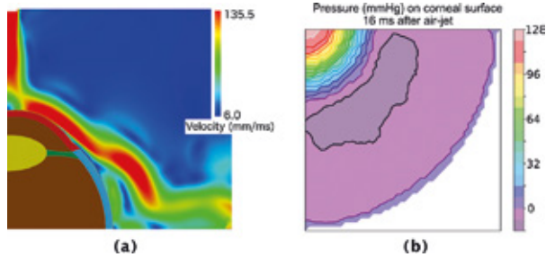
Fluid-structure simulation of the air-puff used to deform the cornea during non-contact tonometry. The fluid velocity on the deformed corneal surface (a) induces a complex distribution of air pressure on the cornea surface (b).
