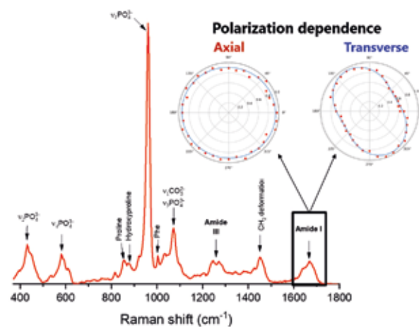
Typical Raman spectrum of bone tissue. The amide I peak is highly polarization dependent, which allows tracking local fibril orientation in 3D. Collaboration with Prof. M. Calame, Empa.
