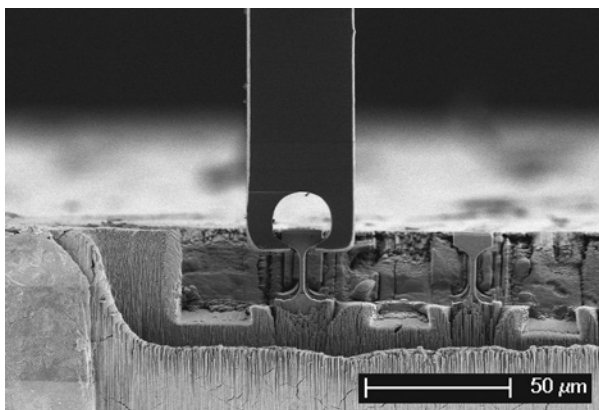
Microtensile experiment on bone tissue. Performing tensile experiments on the length scale of a few μm provides important insights into the properties of nanocomposites such as the bone extracellular matrix.
